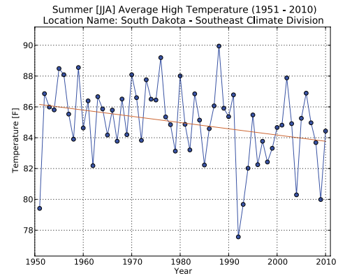
Figure 6. Region-wide temperature trends across Southeast South Dakota from 1951 to 2010 for summer daily maximum temperature (right), summer daily minimum temperature (below left), winter daily maximum temperature (below center), and winter daily minimum temperature (below right)
