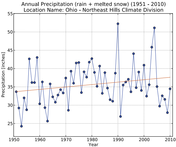
Figure 1 - Average annual precipitation across Northeast Hills Ohio from 1951 to 2010
