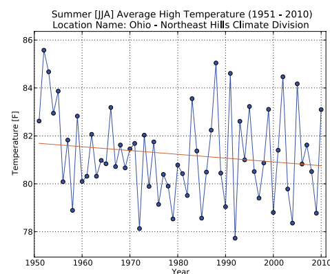
Figure 6. Region-wide temperature trends across Northeast Hills Ohio from 1951 to 2010 for summer daily maximum temperature (right), summer daily minimum temperature (below left), winter daily maximum temperature (below center), and winter daily minimum temperature (below right)
