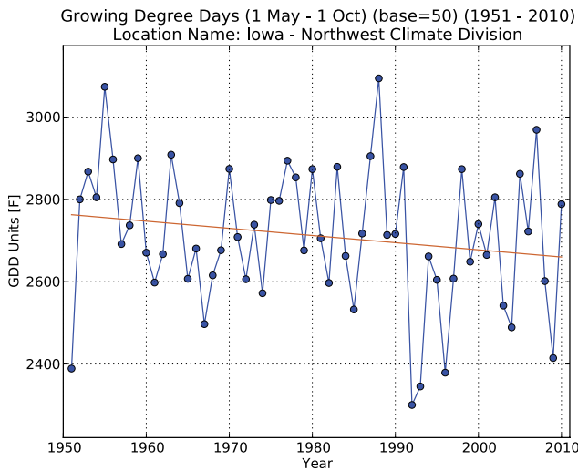
Figure 4 - Number of growing degree days from May 1 to October 1 across Northwest Iowa from 1951 to 2010
