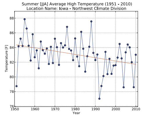
Figure 6. Region-wide temperature trends across Northwest Iowa from 1951 to 2010 for summer daily maximum temperature (right), summer daily minimum temperature (below left), winter daily maximum temperature (below center), and winter daily minimum temperature (below right)
