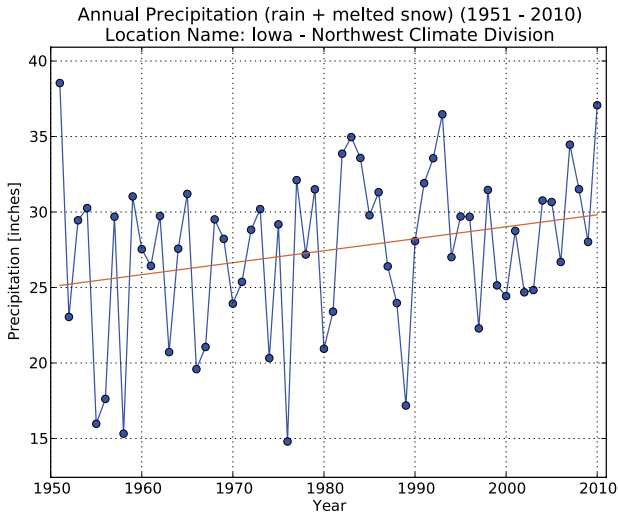
Figure 1 - Average annual precipitation across Northwest Iowa from 1951 to 2010
