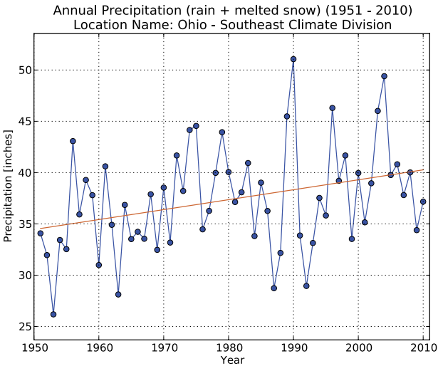
Figure 1 - Average annual precipitation across Southeast Ohio from 1951 to 2010
