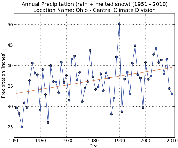
Figure 1 - Average annual precipitation across Central Ohio from 1951 to 2010
