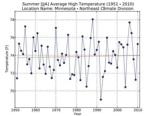
Figure 6. Region-wide temperature trends across Northeast Minnesota from 1951 to 2010 for summer daily maximum temperature (right), summer daily minimum temperature (below left), winter daily maximum temperature (below center), and winter daily minimum temperature (below right)
