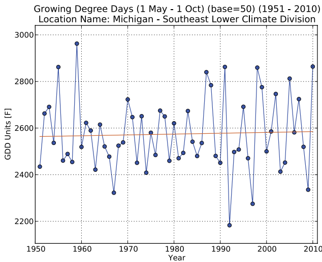
Figure 4 - Number of growing degree days from May 1 to October 1 across Southeast Lower Michigan from 1951 to 2010
