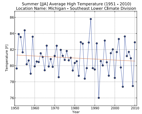
Figure 6. Region-wide temperature trends across Southeast Lower Michigan from 1951 to 2010 for summer daily maximum temperature (right), summer daily minimum temperature (below left), winter daily maximum temperature (below center), and winter daily minimum temperature (below right)
