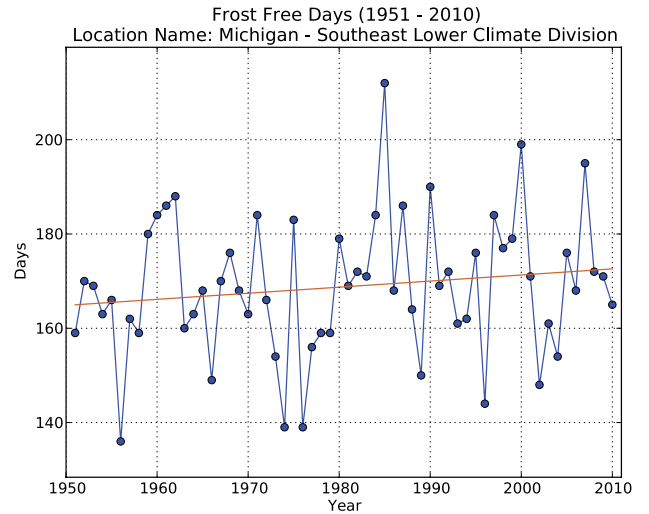
Figure 3 - Number of frost-free days across Southeast Lower Michigan from 1951 to 2010
