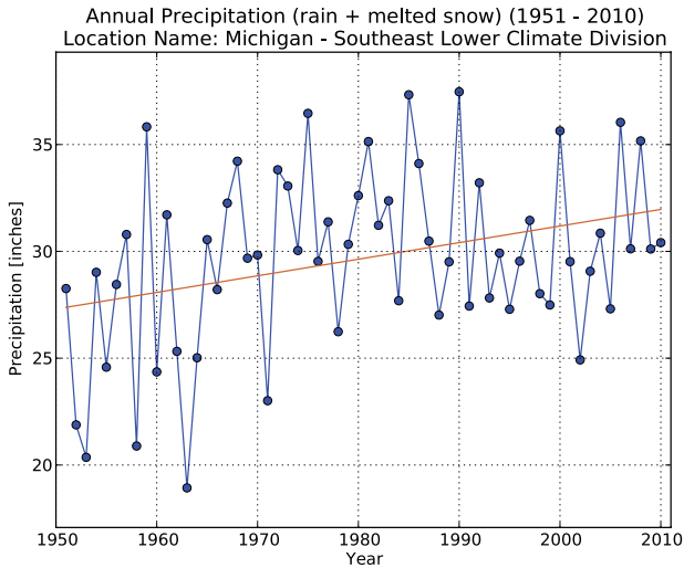
Figure 1 - Average annual precipitation across Southeast Lower Michigan from 1951 to 2010
